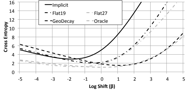
Figure 2: Cross-entropy of various priors and the oracle prior as a function of calibration shift. Priors in gray utilize oracle information.
